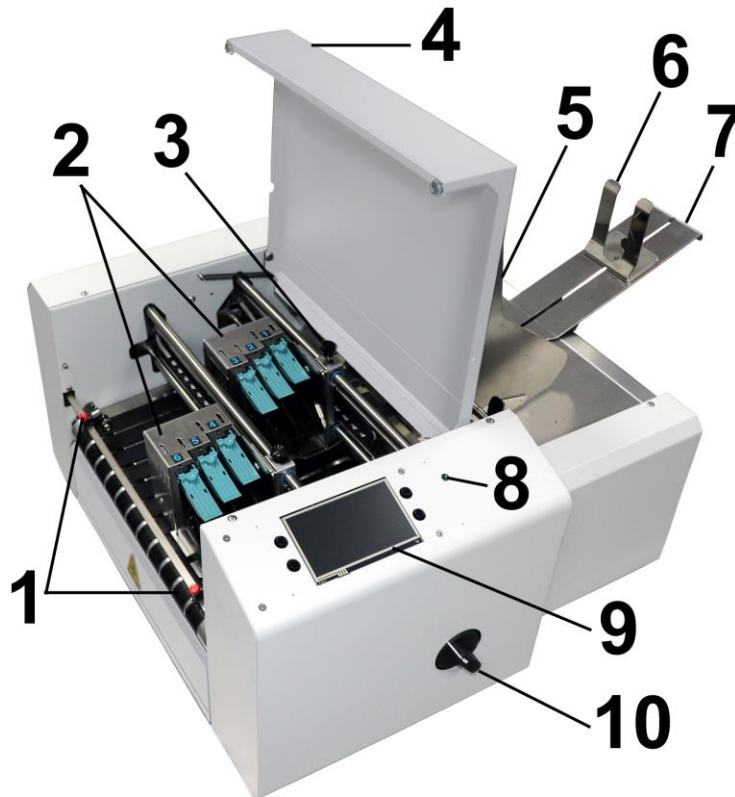
Operator View
